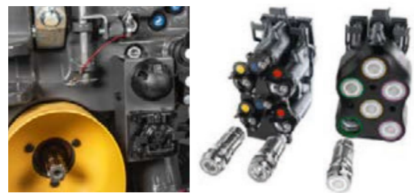
At the front, the Fendt 900 Vario offers the option of an integrated power lift with position and load relief control. You can also have up to two front valves with a flow volume of up to 100 l/min, a front PTO and an ISOBUS plug.
